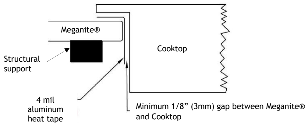
Heat Reflective Tape Illustration
